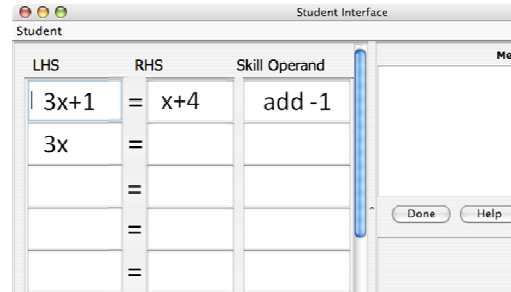
Fig. 1. The Tutor Interface for the Algebra I CTAT Tutor. Students are supposed to enter an operation for transformation first in the column labeled as “Skill Operand.” Then corresponding expressions for the left- and right-hand sides must be entered.
